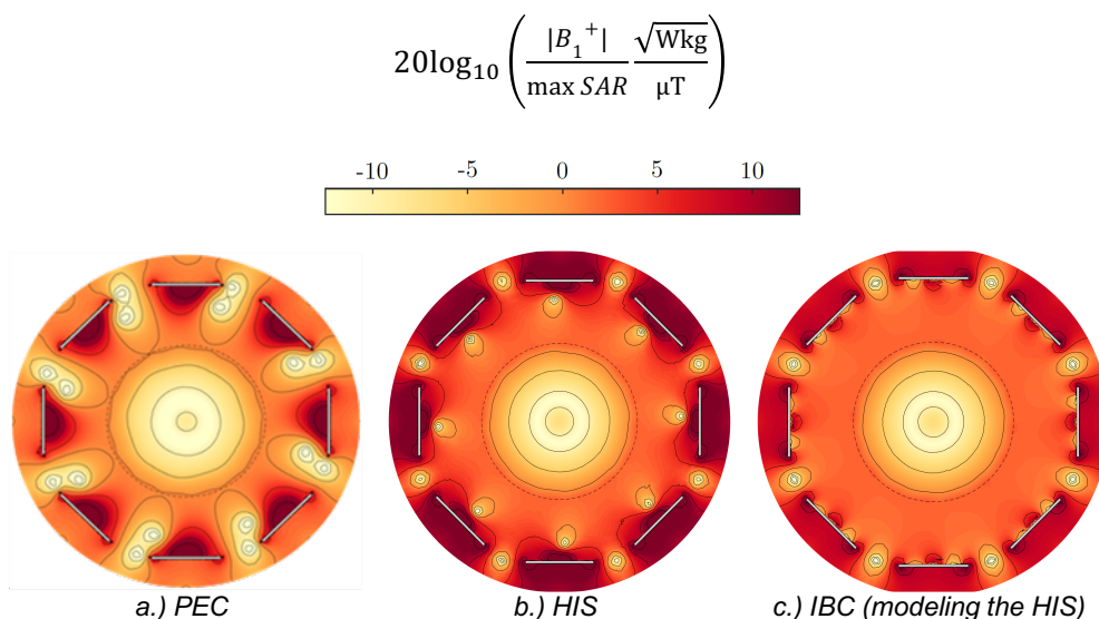
Fig.1: Magnetic flux density |B_1^+| normalized to the maximum of the SAR inside the homogeneous tissue for different shield types. a.) conventional PEC shield, b.) HIS shield and c.) Impedance boundary condition modeling the HIS. The tissue is denoted by the dotted line.
